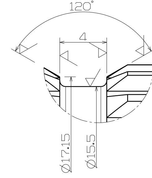
DETAIL "C" (5:1)
