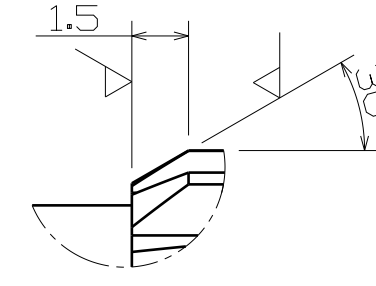
DETAIL "B" (5:1)
